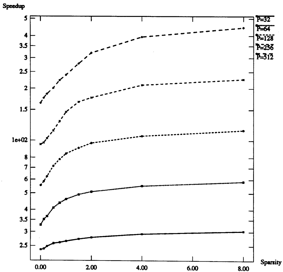
Figure 8: Speedup vs. Sparsity
