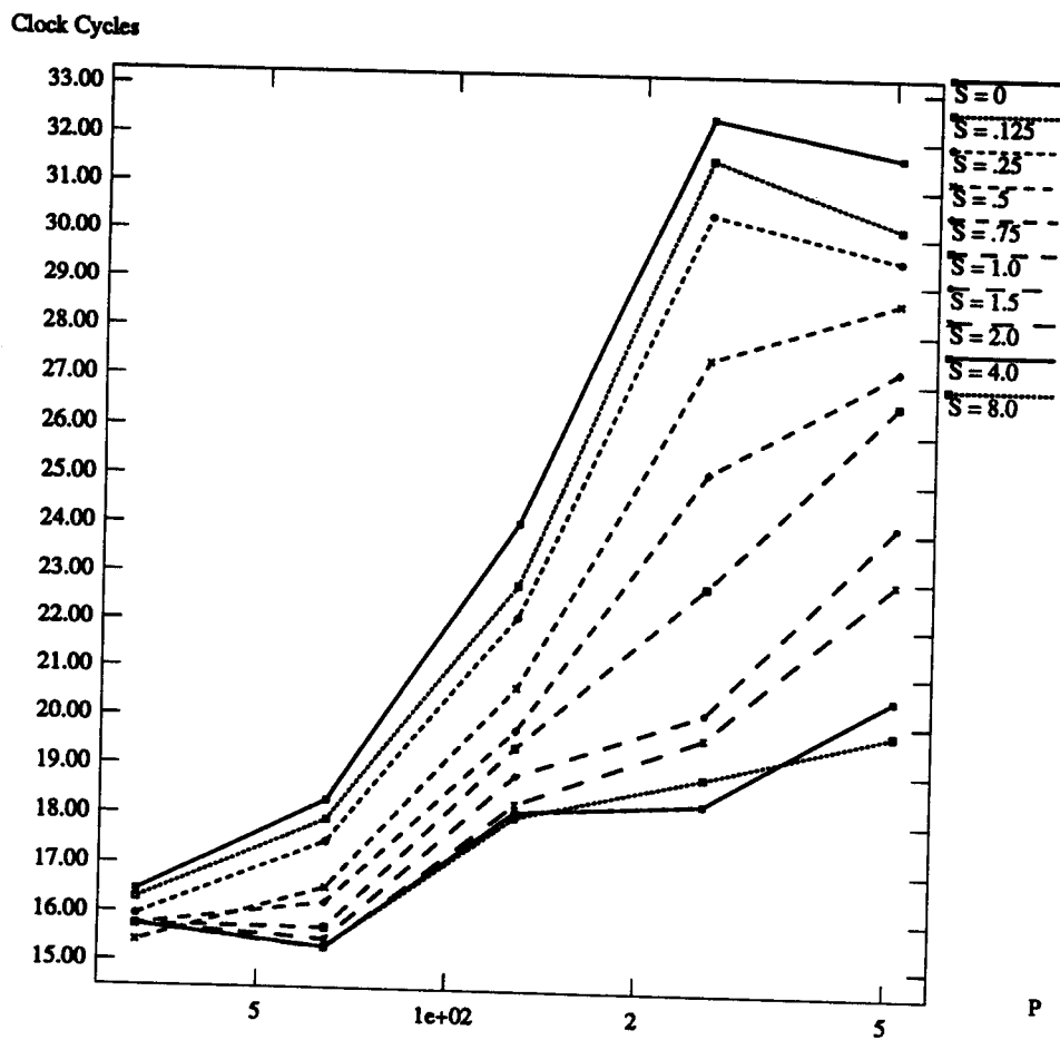
Figure 10: Block Latency vs. System Size
