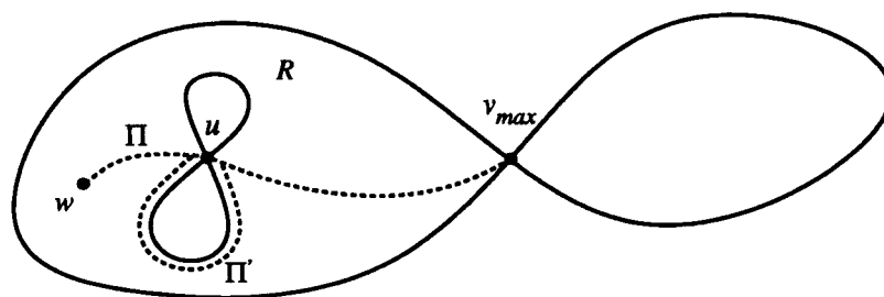
Figure 2: Illustration of the proof of Lemma 3.1.
