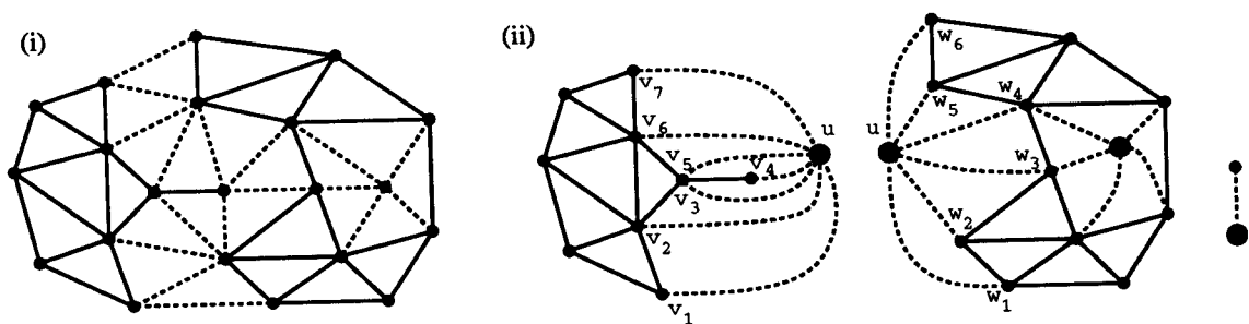
Figure 6: (i) A terrain F that is split by a path of edges and a cycle of edges (dashed) into three components. (ii) The three components and how they are restored.
