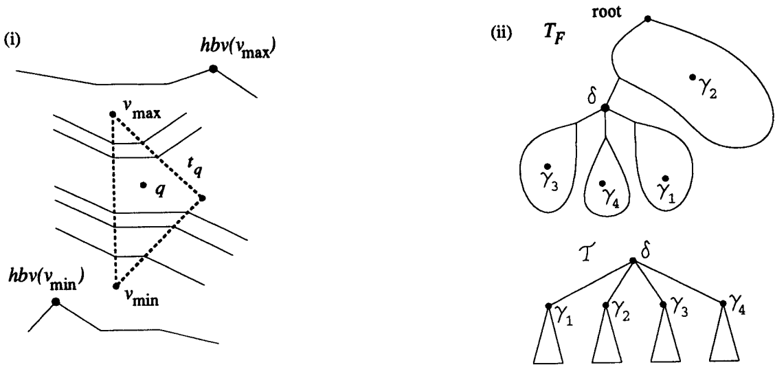
Figure 4: (i) The triangle t_q in a part of the height level map, and the vertices hbv(v_{\max}) and hbv(v_{\min}) . (ii) Deciding in which subtree below \delta to continue by means of lowest common ancestor queries in T_F .
