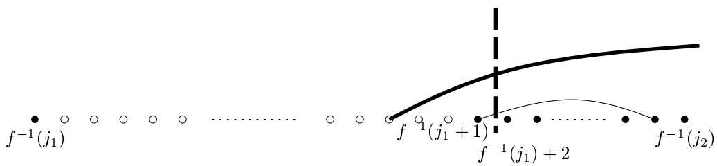
Figure 5: Illustration with the proof of Lemma 6
