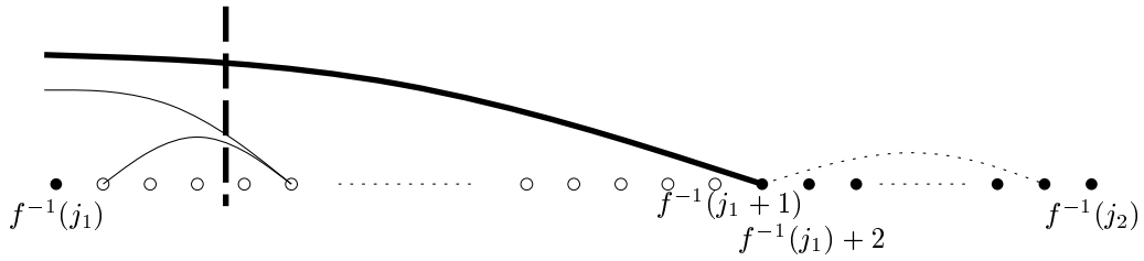
Figure 4: Illustration with the proof of Lemma 6
