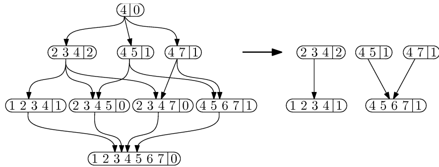
Figure 4: The intersection structure for \{\{1, 2, 3, 4\}, \{2, 3, 4, 5\}, \{4, 5, 6, 7\}, \{2, 3, 4, 7\}\} (with the demands next to the sets) and the corresponding connectivity structure.
