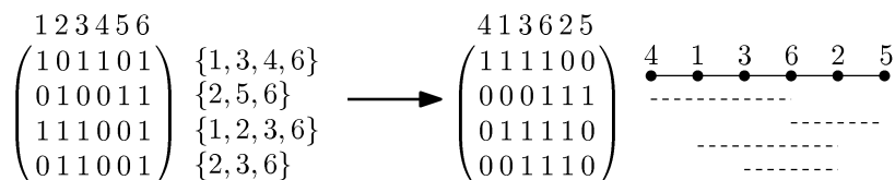
Figure 2: Finding a path support via the consecutive ones property.
