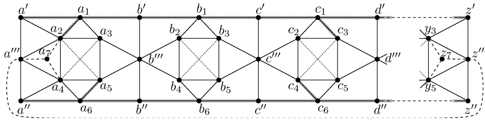
Figure 8: Construction of a hypergraph and its planar/2-outerplanar support from a 3-SAT instance.
