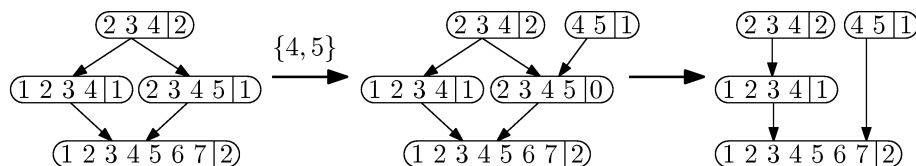
Figure 5: Incremental construction of the connectivity structure.
