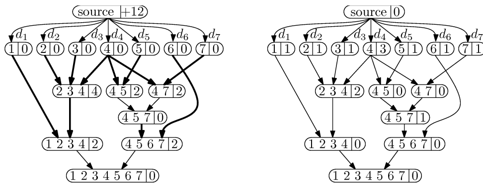
Figure 6: The original (left) and the new (right) flow network. Thick edges denote a lower bound on the flow. In the flow networks the production/consumption (left) or the capacity to the sink (right) is shown instead of the demand.
