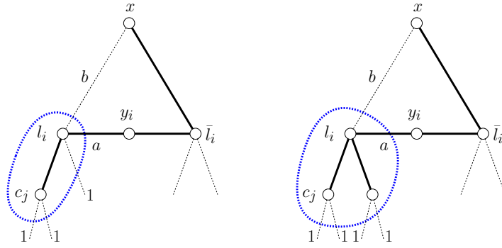
Figure 4: Unsatisfied clauses.
