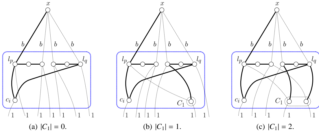
Figure 3: The cases of |C_1| \leq 2 .
