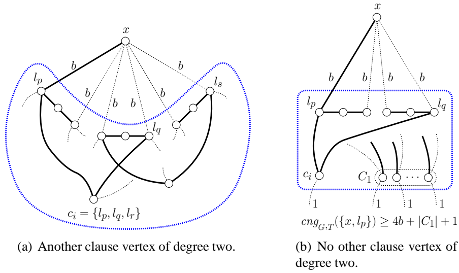
Figure 2: A clause vertex c_i of degree two.
