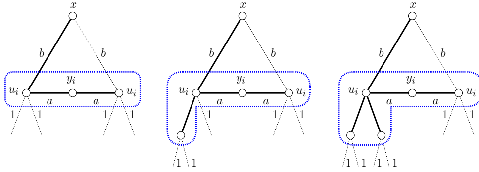
Figure 5: A spanning tree of congestion at most k .
