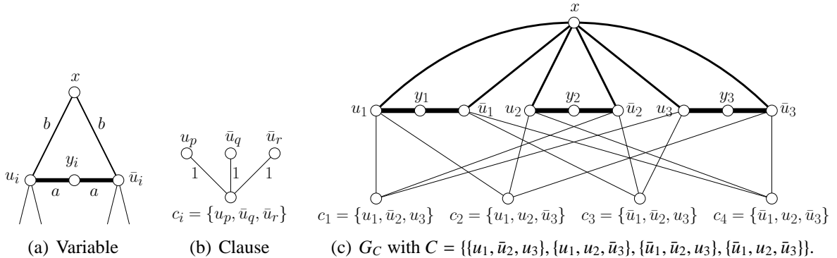
Figure 1: Gadgets, and a constructed graph.
